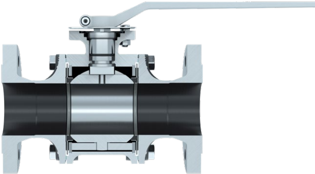
Trunnion mounted (TM)
