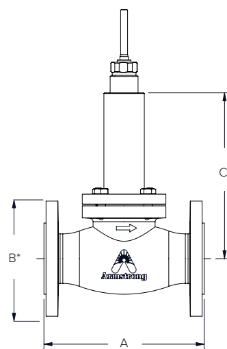
Bellow Seal - Cryogenic** - LeakOff** Bonnet
